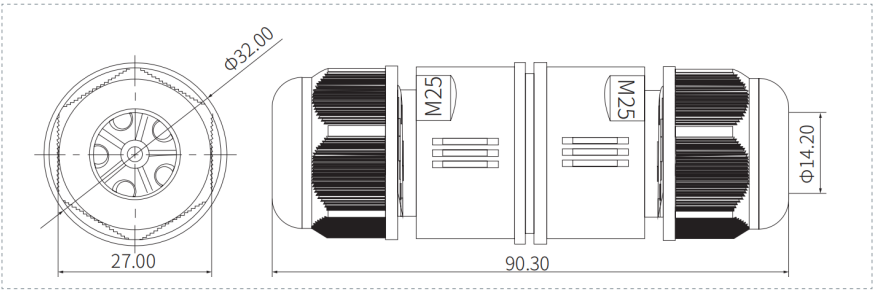
尺寸图 /Dimensional drawing
