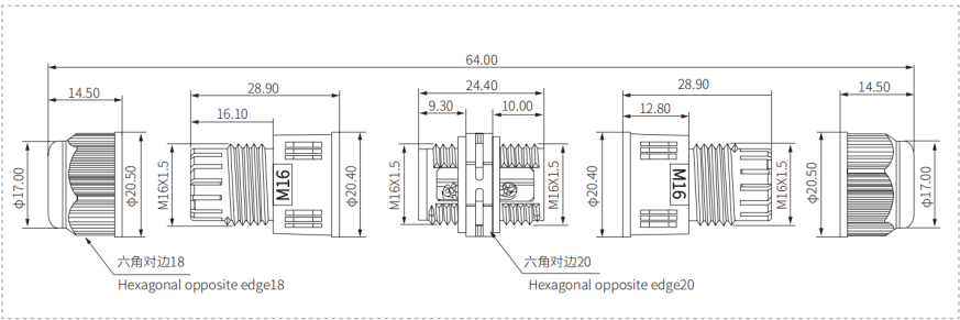
尺寸图 /Dimensional drawing
